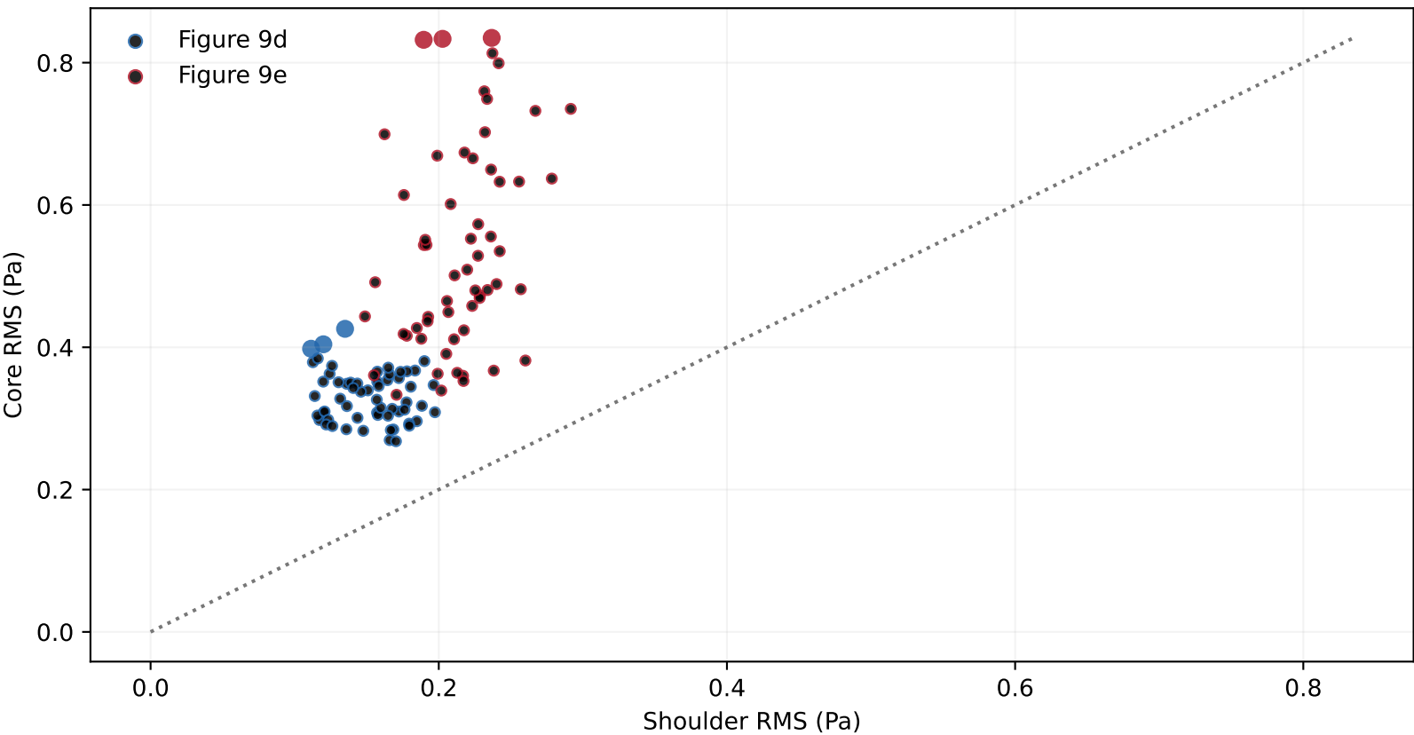
C. Pulse-core RMS against local-cycle shoulders
